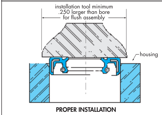
PROPER INSTALLATION
