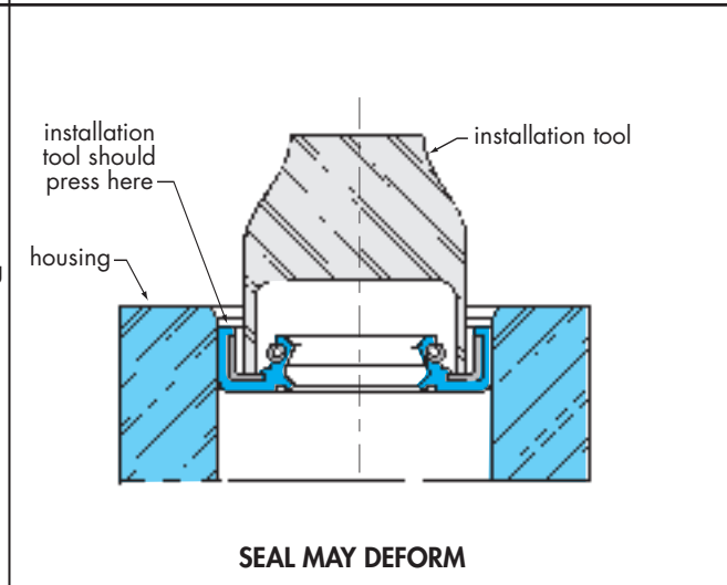
DEFORMED SEAL
