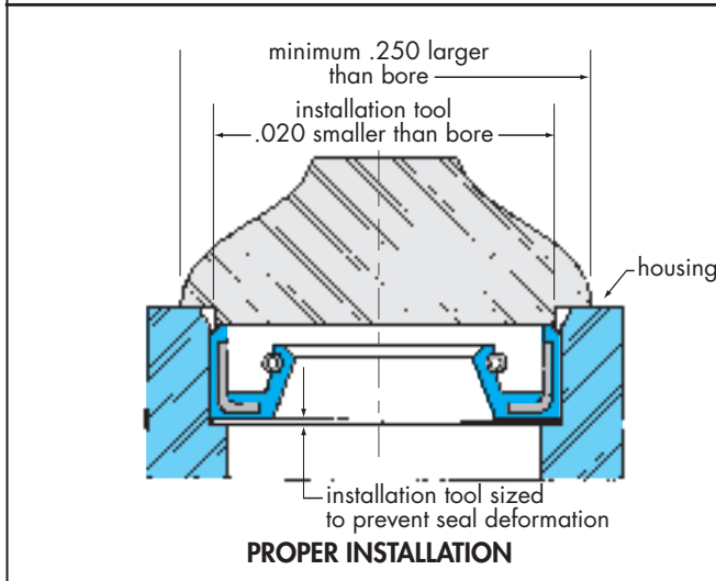
PROPER INSTALLATION
